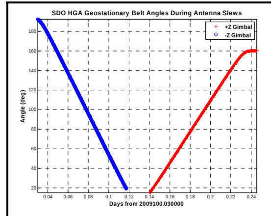
Figure 7. Clarke Belt Intersection Angle
